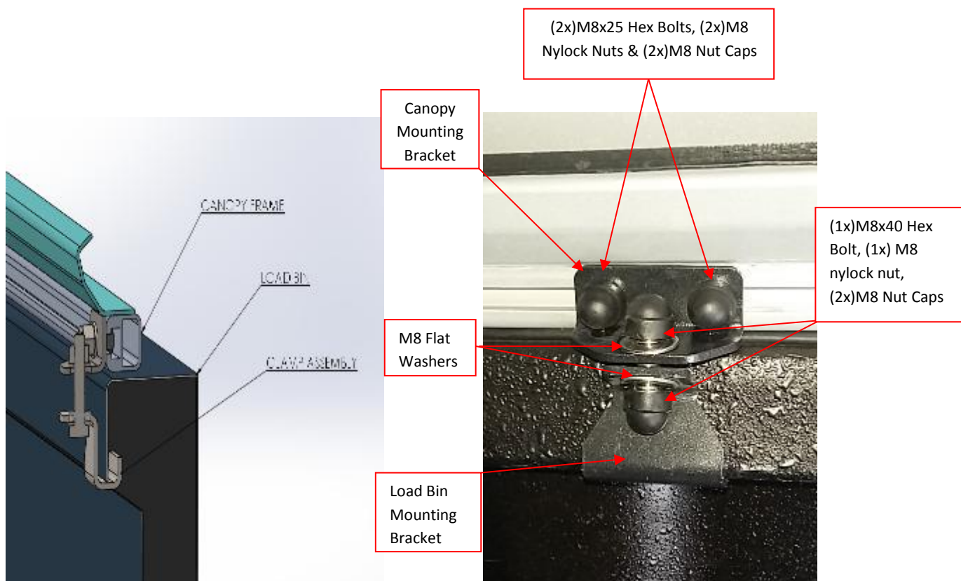
Figure 10: Centre Bracket Mounting Assembly
